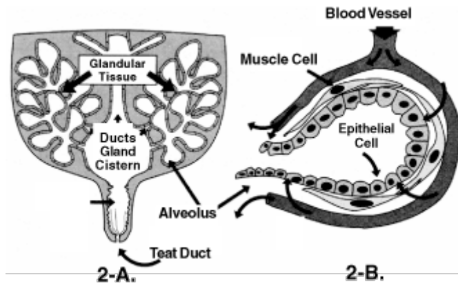
Figure 2. Structure of the mammary gland showing teat and gland cisterns, milk ducts, and glandular tissue (A). Glandular tissue is made up of many small microscopic sacs called alveoli that are lined by milk-producing epithelial cells (B). There are millions of alveoli within each mammary gland.
